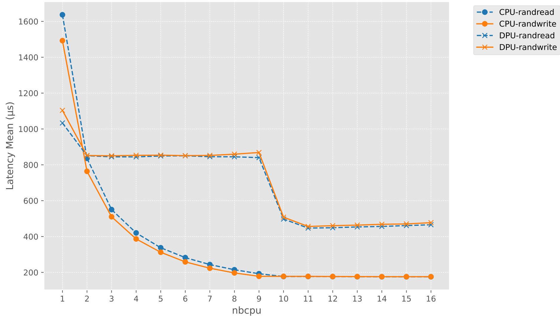
Latency Mean vs nbcpu
